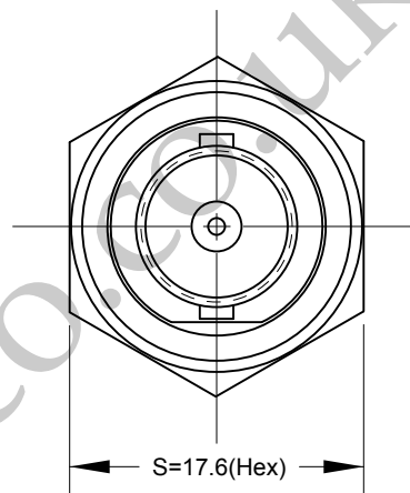
End View Nut, Washer and Neoprene removed.
