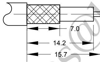
Cable Preparation
