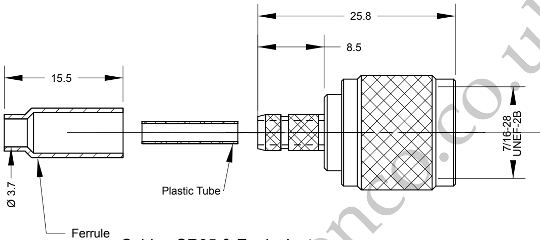
Cable : SR35 & Equivalents
