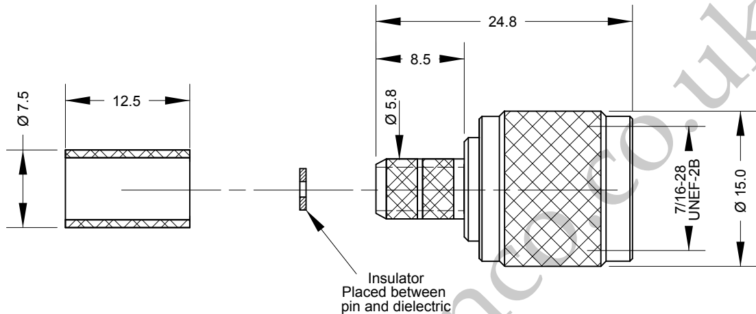
Cable : RG8Mini, ANT240, LMR240 & Equivalents
