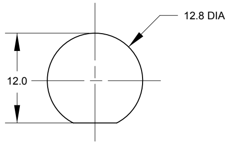
Panel Mounting Hole Cutout
